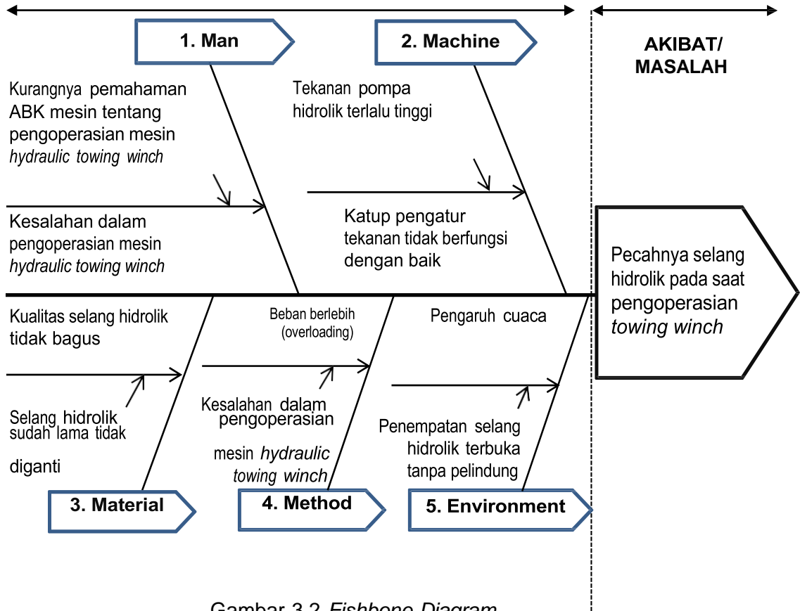
Gambar 3.2 Fishbone Diagram
