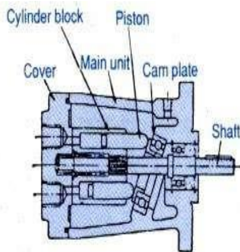
Gambar 2.9 Axial Plunger Hydraulic Motor
