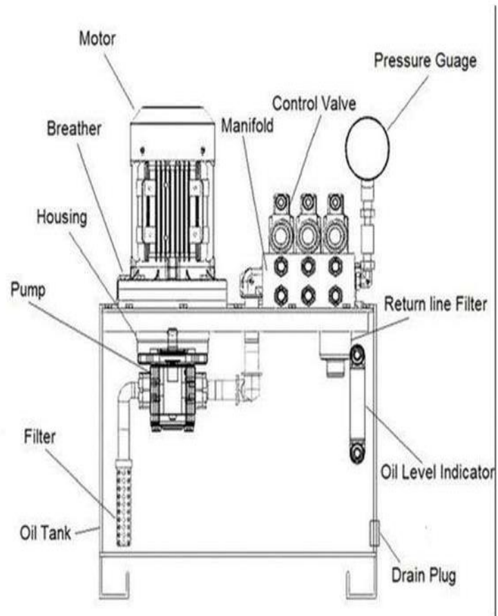
Gambar 2.2 Hydraulic Power Pack
