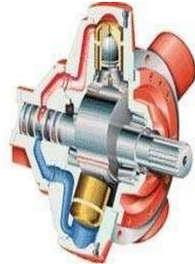
Gambar 2.10 Radial Piston Hydraulic Motor
